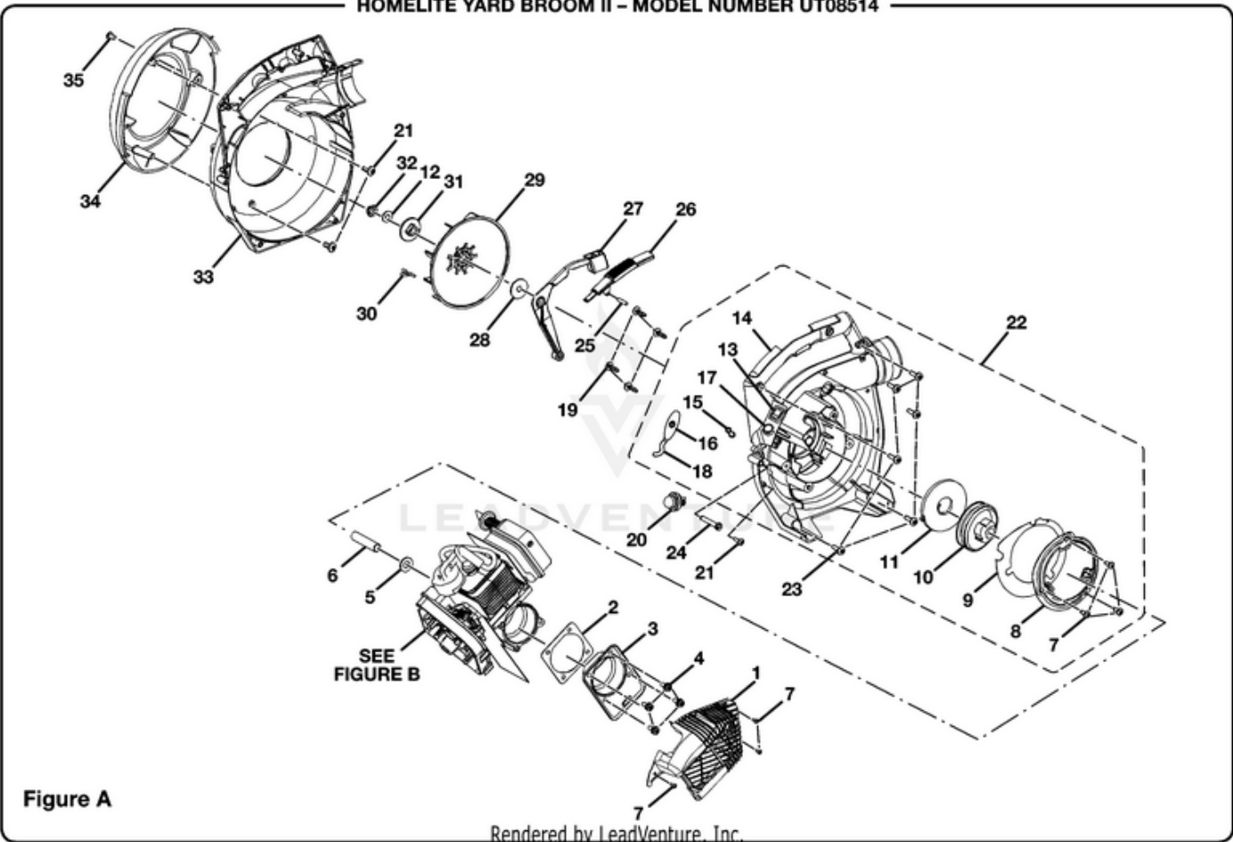
Vac Attack II Blower UT-08514 - Figure A
