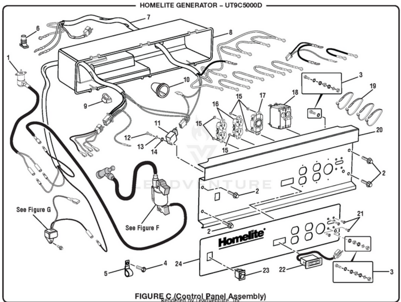
UT9C5000D 5000 Watt Generator - Figure C (Control Panel Assembly)
