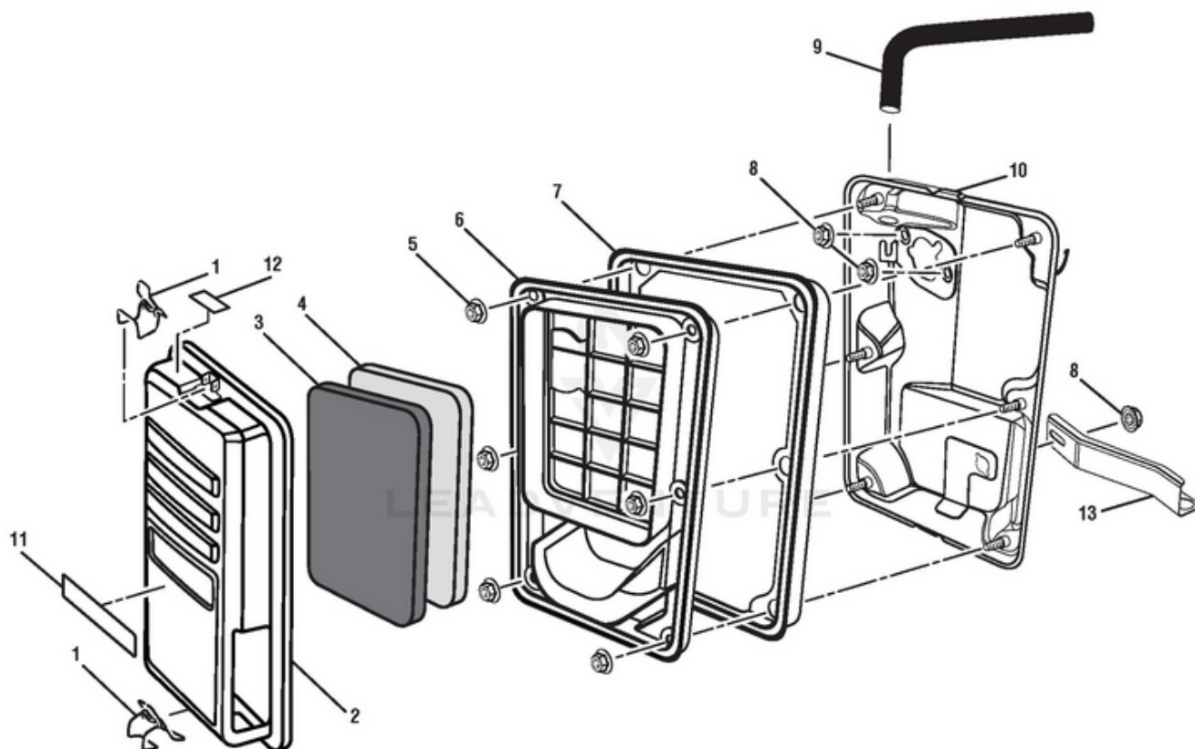
FIGURE L (Air Cleaner Assembly)
