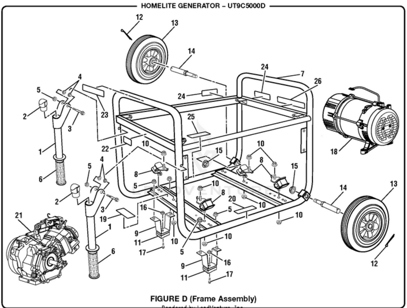
UT9C5000D 5000 Watt Generator - Figure D (Frame Assembly)
