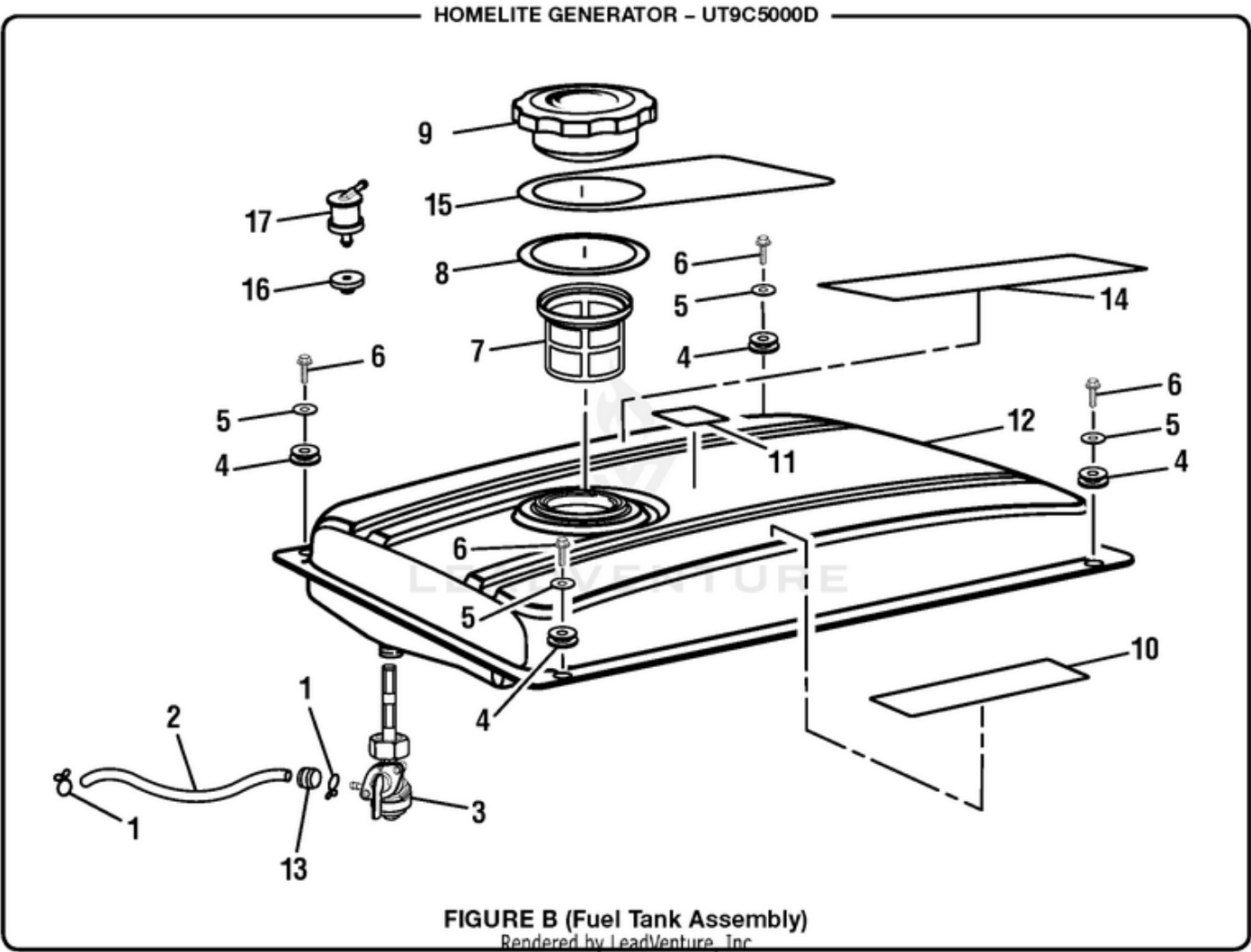
UT9C5000D 5000 Watt Generator - Figure B (Fuel Tank Assembly)
