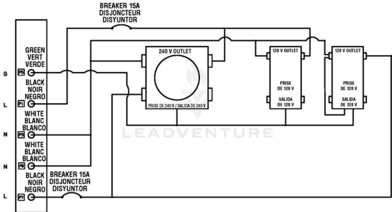
WIRING DIAGRAM SCHÉMA DE CÂBLAGE / DIAGRAMA DE CABLEADO Rendered by LeadVenture, Inc
