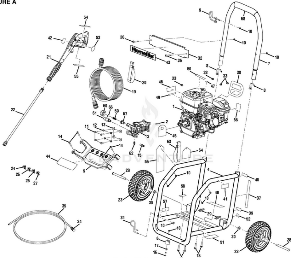
HOMELITE PRESSURE WASHER — MODEL NO. UT80953E
