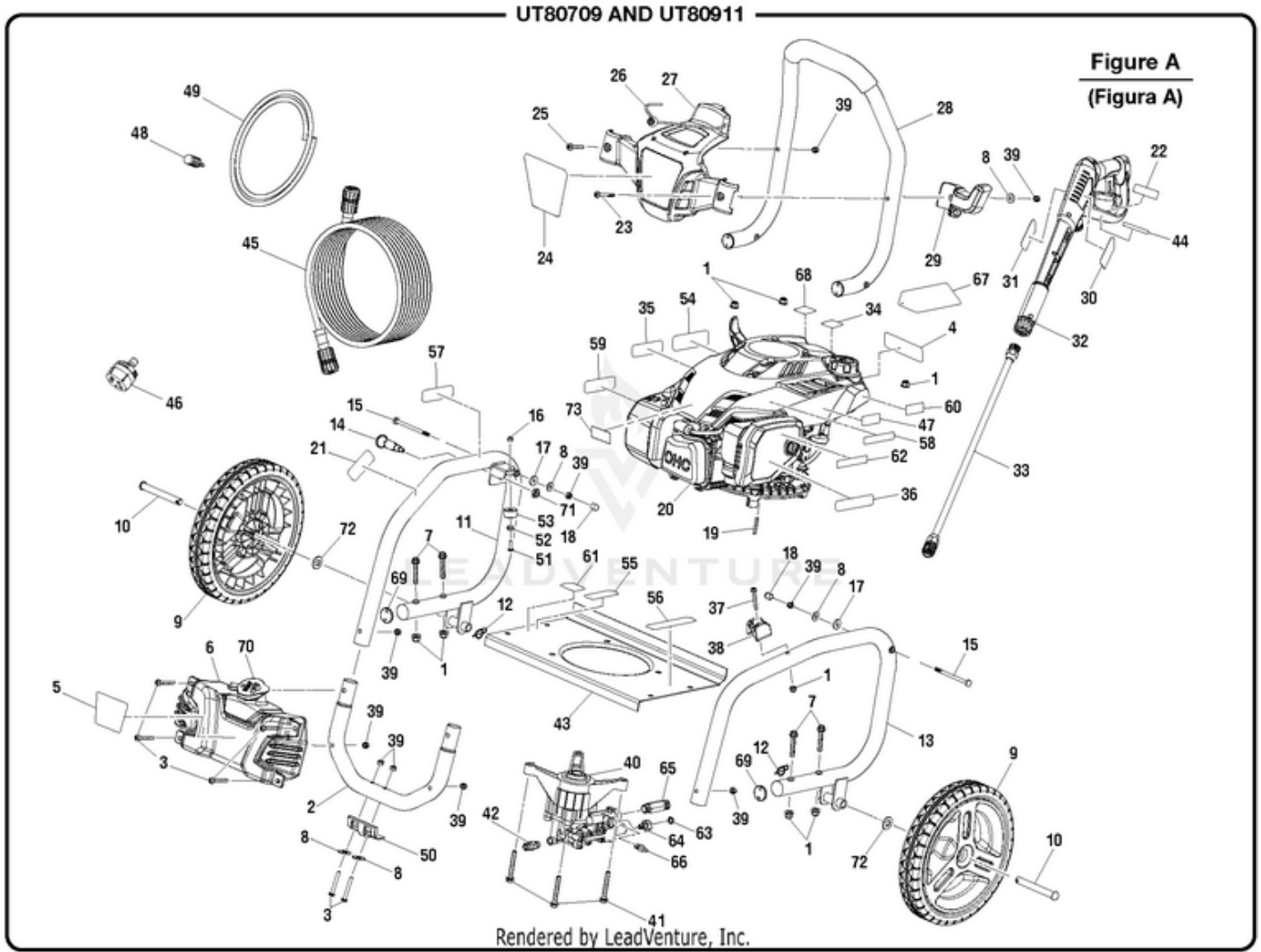
UT80911 Pressure Washer - Figure A
