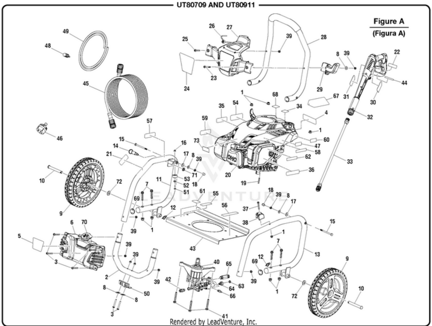
UT80709 Pressure Washer - Figure A
