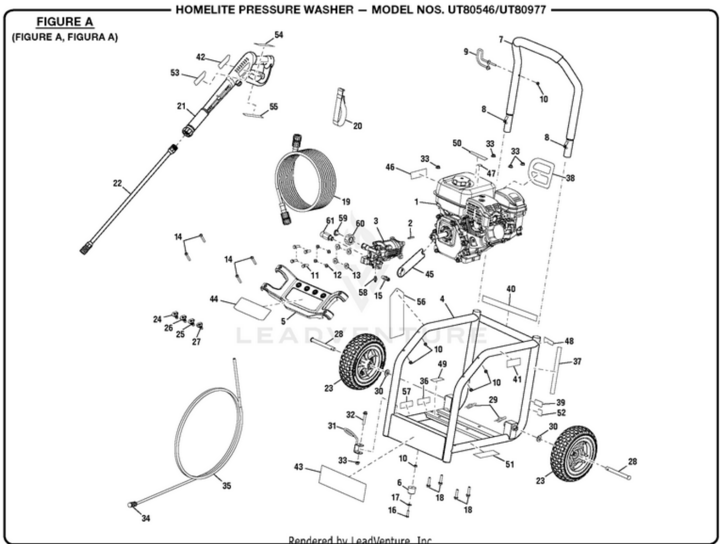
UT80546 Pressure Washer - Figure A
