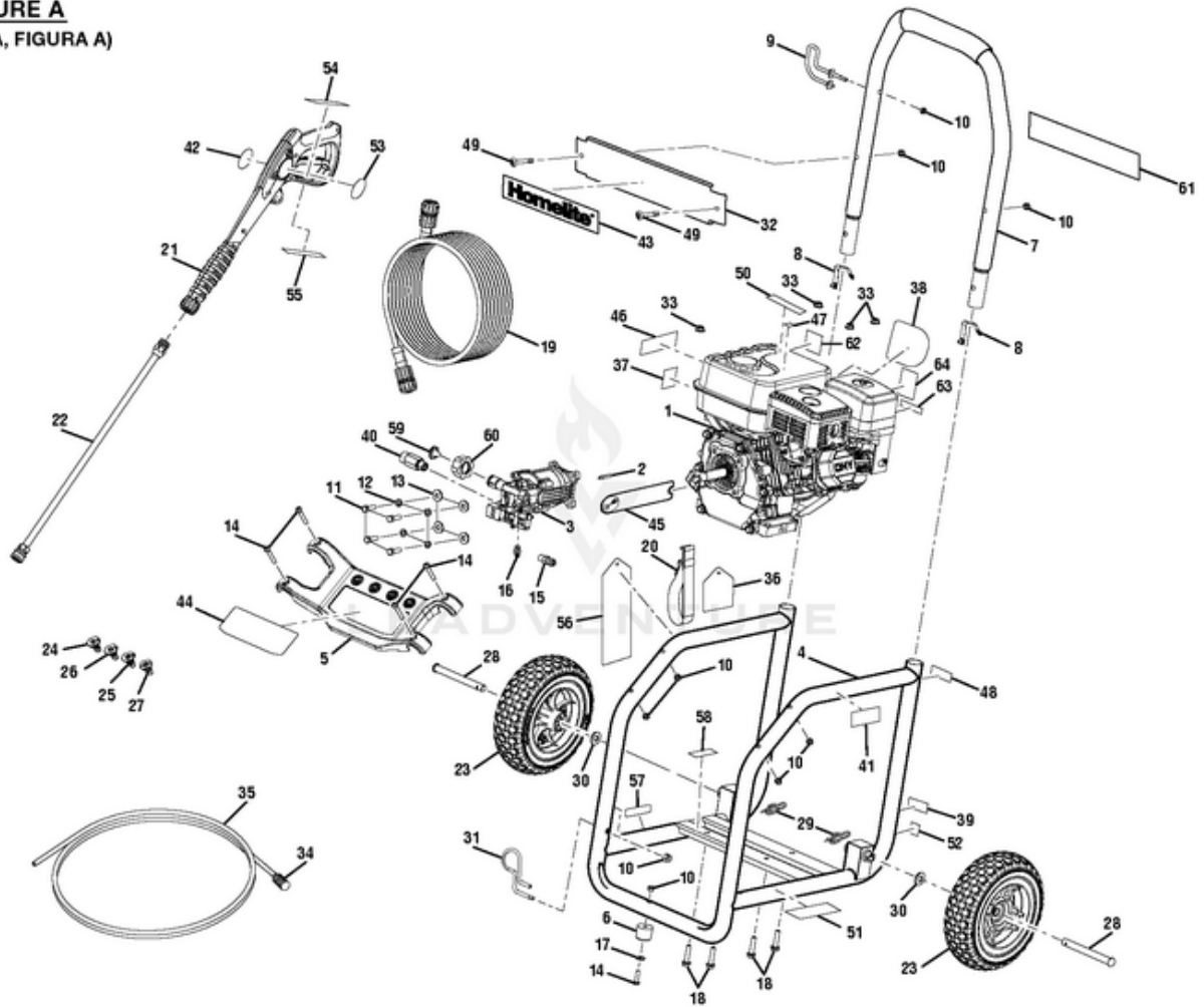
HOMELITE PRESSURE WASHER – MODEL NO. UT80522D
