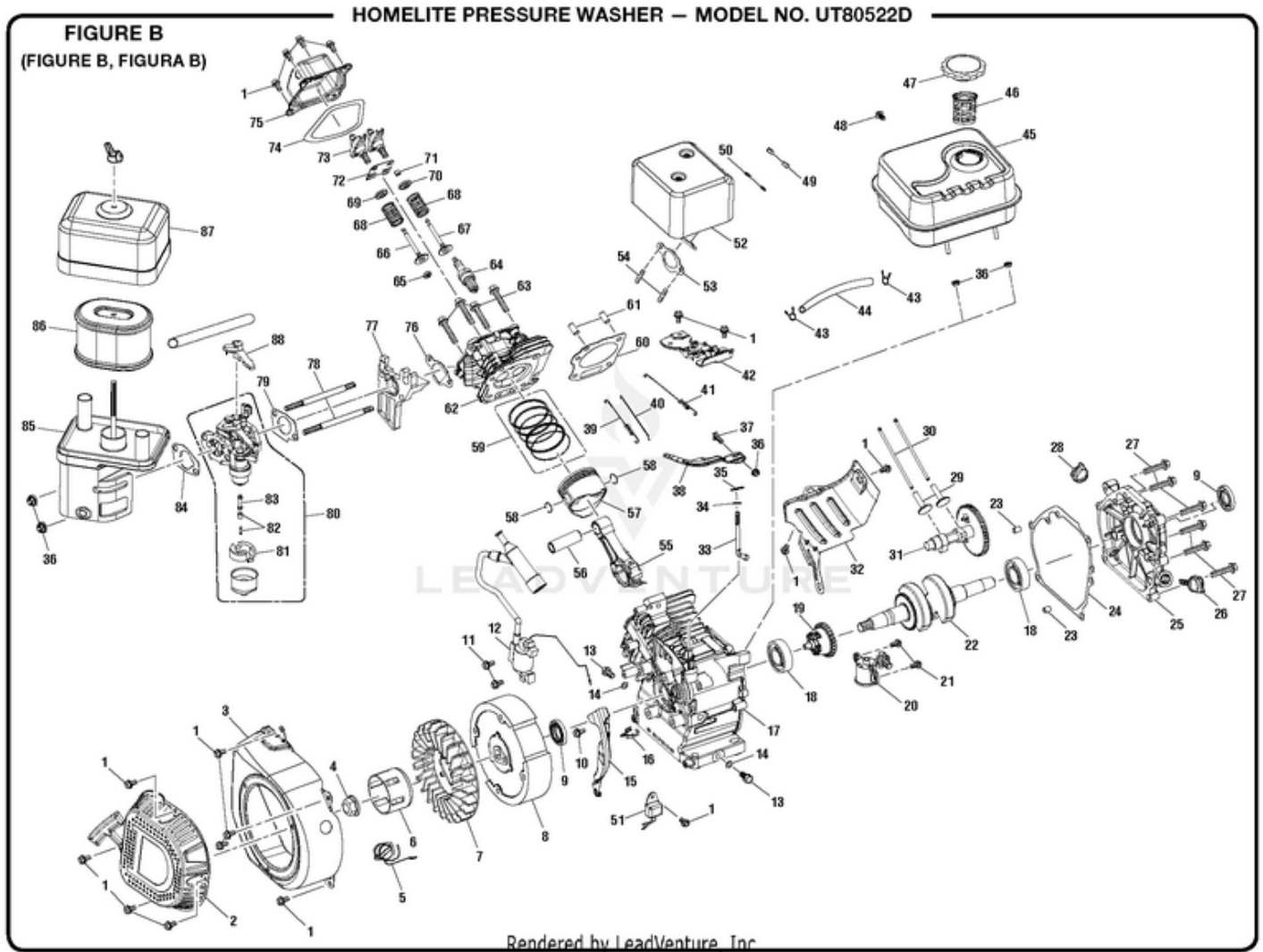
UT80522D Pressure Washer - Figure B
