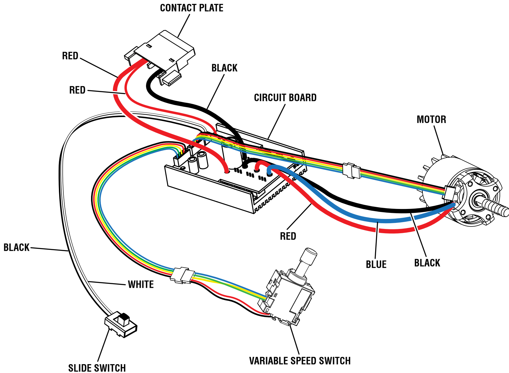
WIRING DIAGRAM
