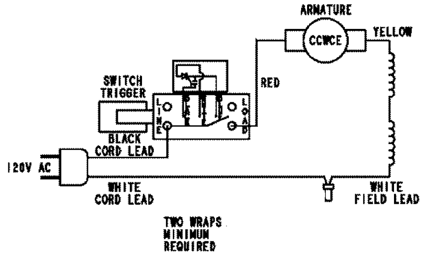
WIRING DIAGRAM 120V VARIABLE SPEED GROUP 1
