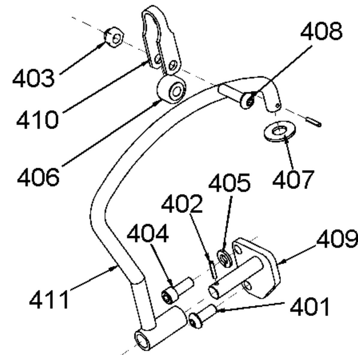
SUSPENSION HANGER ASSEMBLY PART NO. HR-55097
