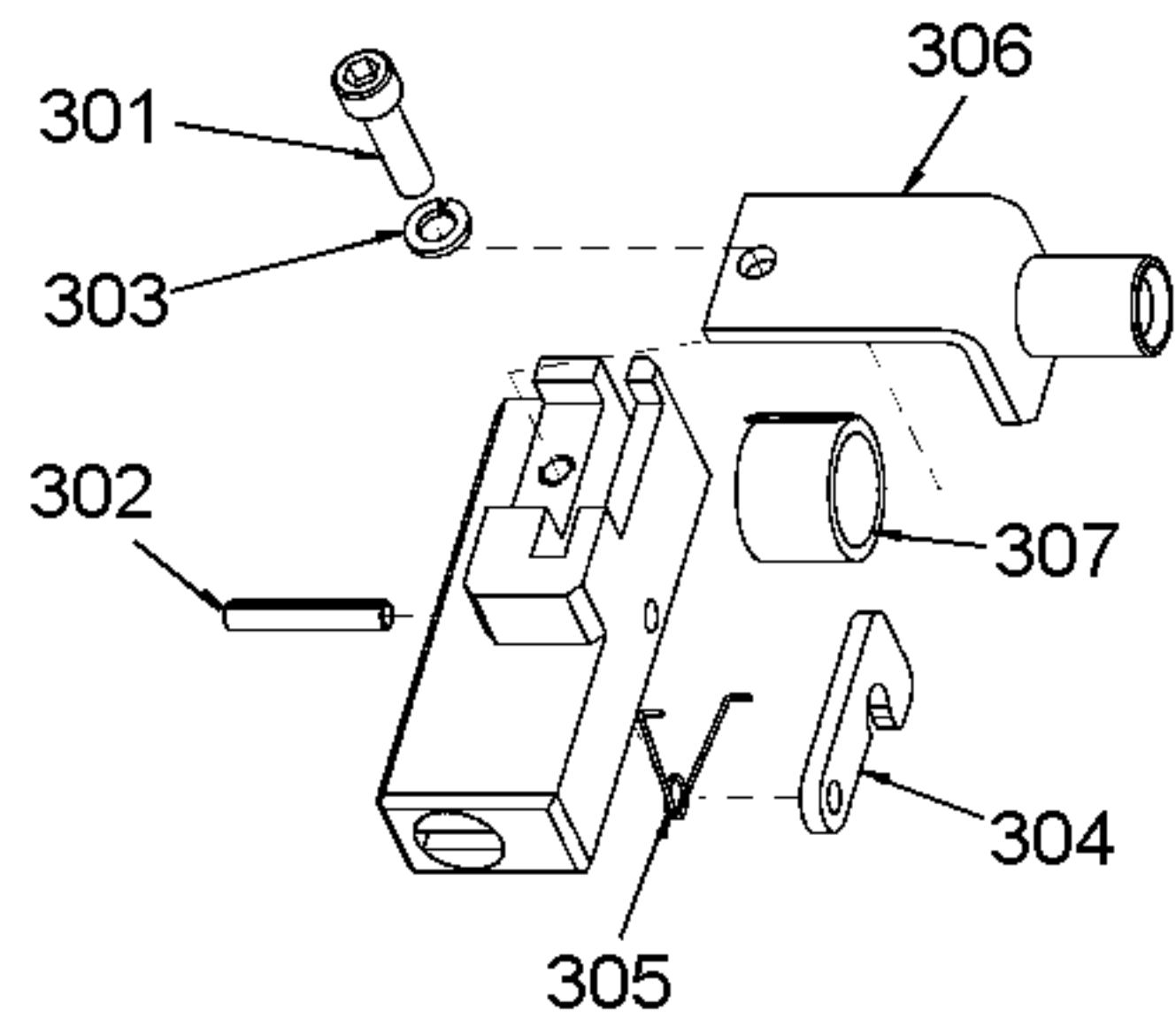
FOLLOWER ASSEMBLY
