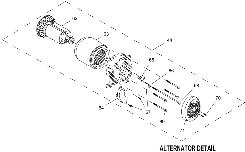
ALTERNATOR DETAIL
