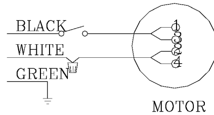
WIRING DIAGRAM (230 VOLT)
