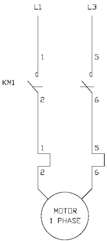
MODEL 50-763 SINGLE PHASE POWER CIRCUIT
