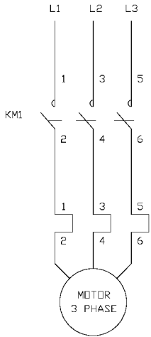
MODEL 50-762 THREE PHASE POWER CIRCUIT
