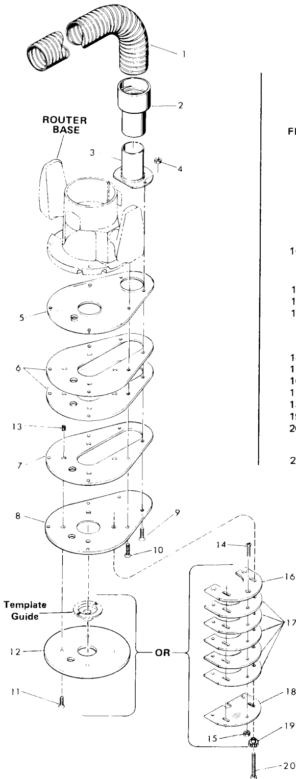
ROUTER CHIP COLLECTOR KIT (Fig. Nos. 1 thru 21)
