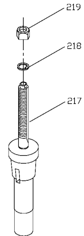
43-802 1/2" SPINDLE
