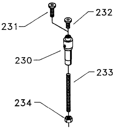
43-144 STUB SPINDLE
