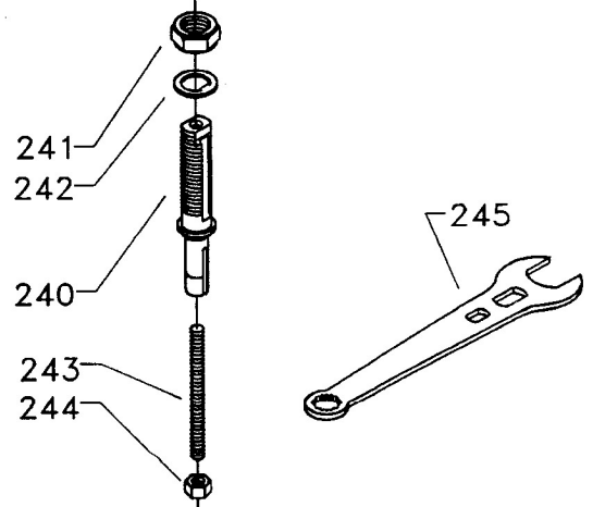
43-143 3/4" SPINDLE ASSEMBLY
