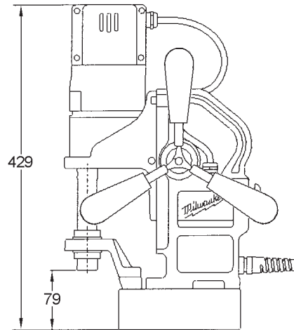
50mm DEPTH OF CUT SET-UP
