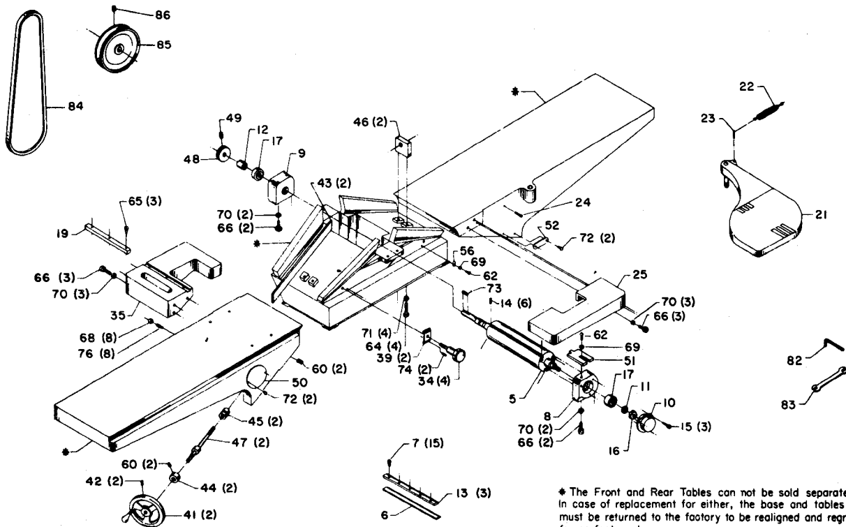
BASE ASSEMBLY
