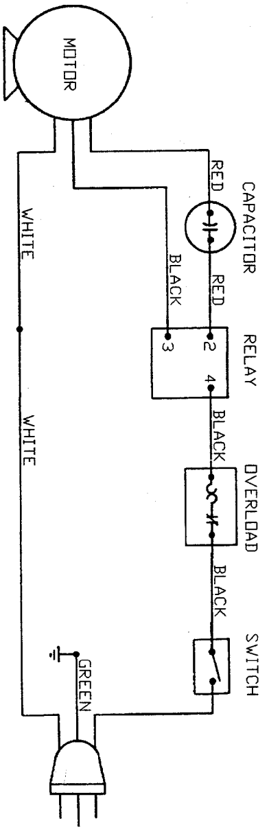
WIRING DIAGRAM
