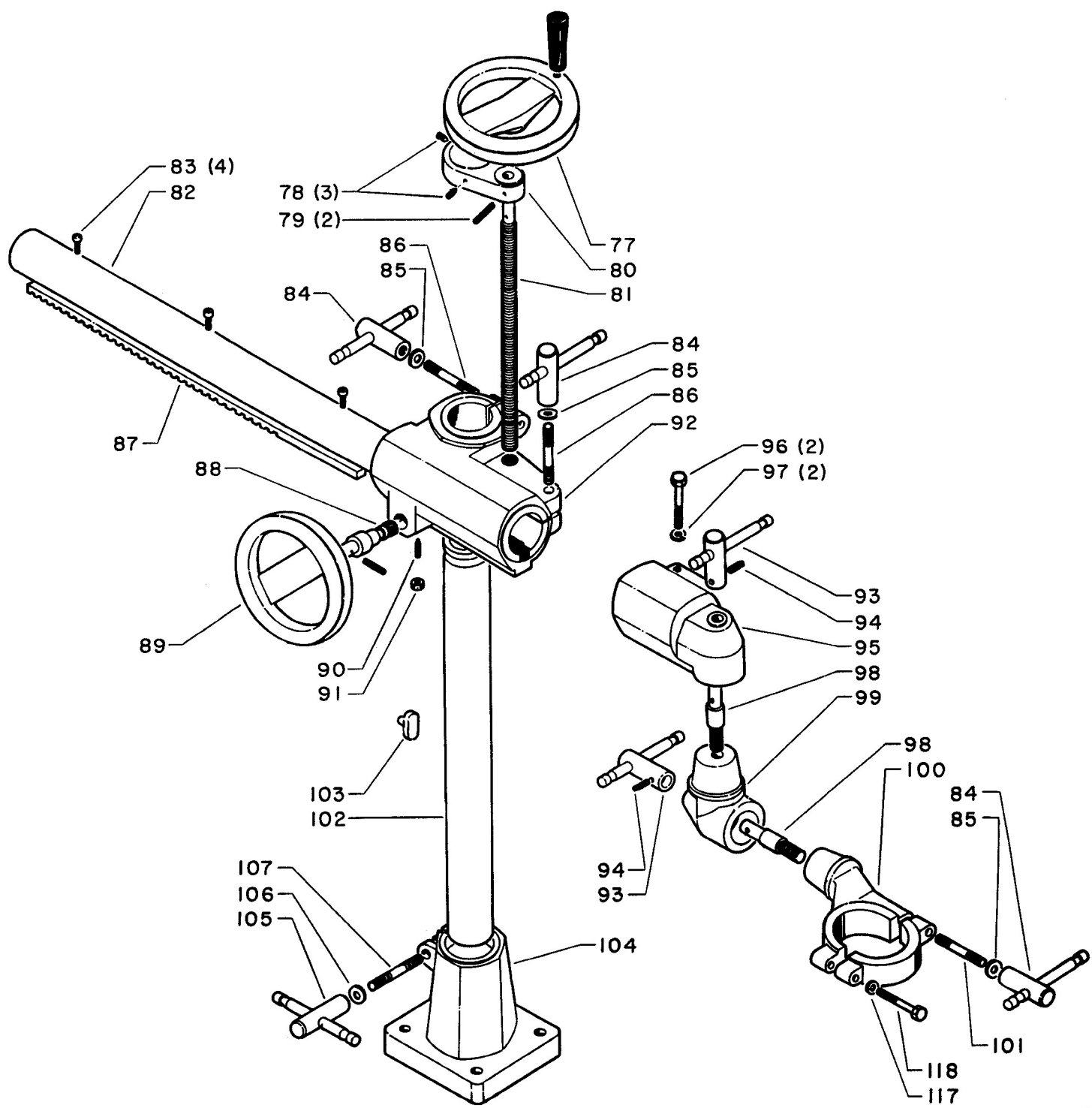
34-996 SUPPORT STAND & 34-990 BASE ASSEMBLY
