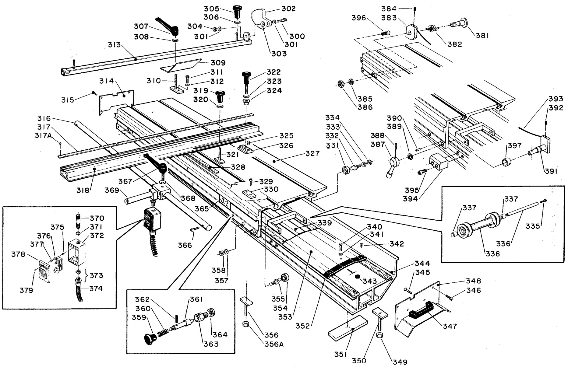
SLIDING TABLE ASSEMBLY
