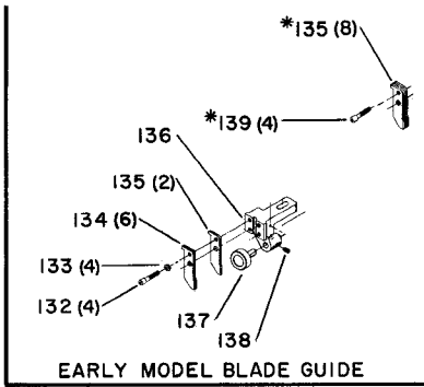
EARLY MODEL BLADE GUIDE
