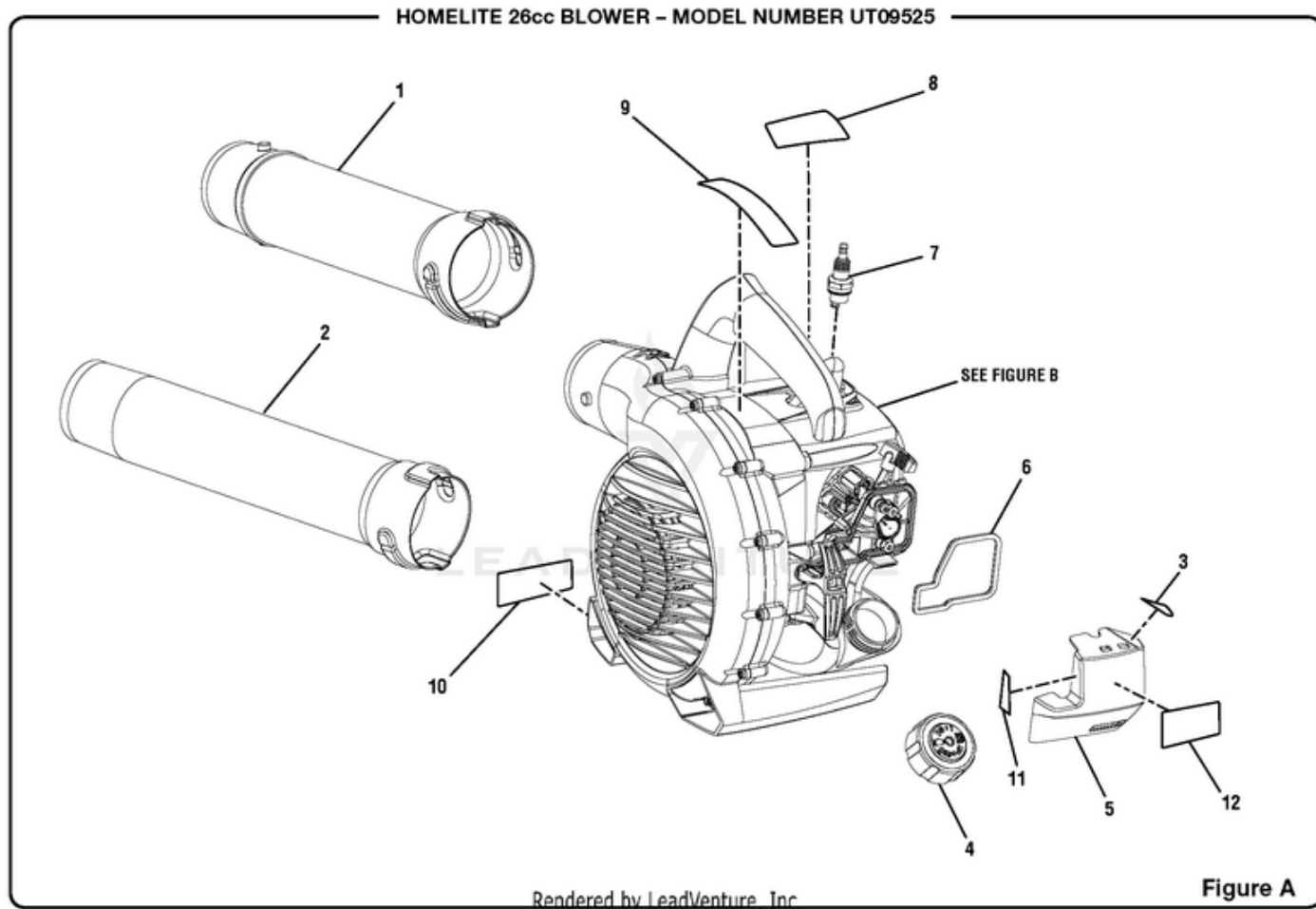
UT09525 26cc Blower - Figure A
