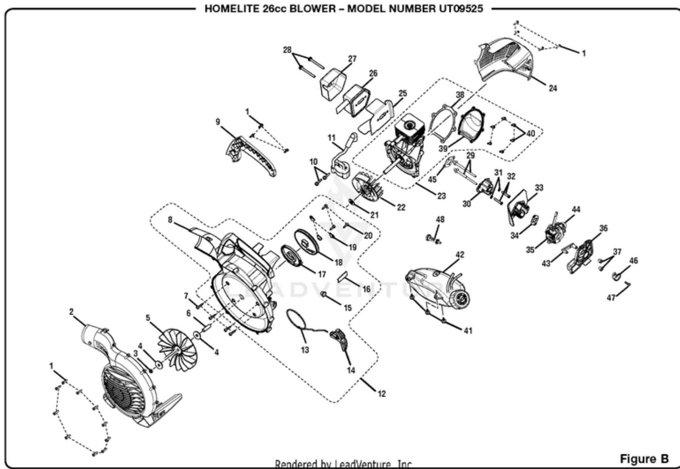
UT09525 26cc Blower - Figure B
