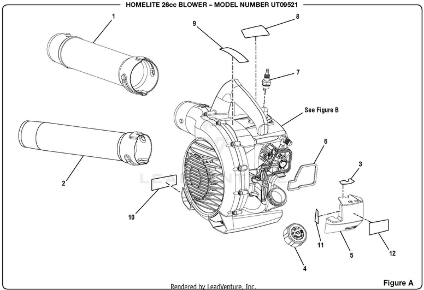
UT09521 26cc Blower - Figure A
